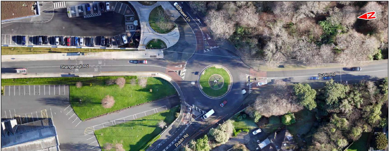
Image 6.39: Shankill Four-Arm Roundabout
