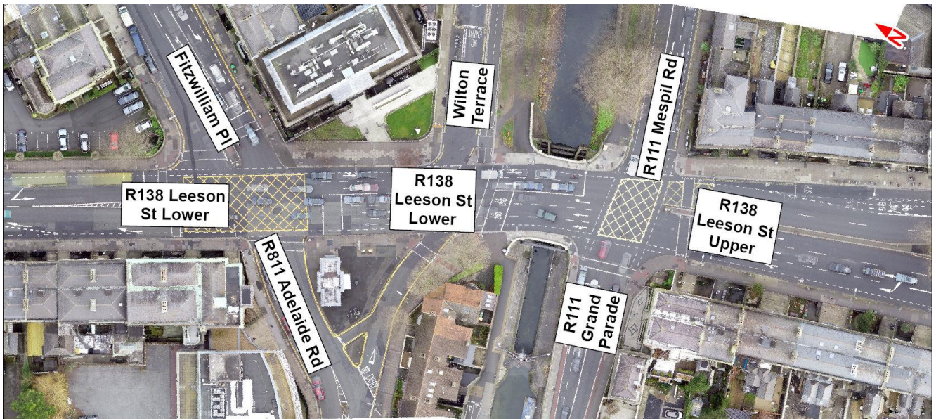
Image 6.3: R138 Leeson Street Lower / Fitzwilliam Place Four-Arm Signalised Junction Arrangement
