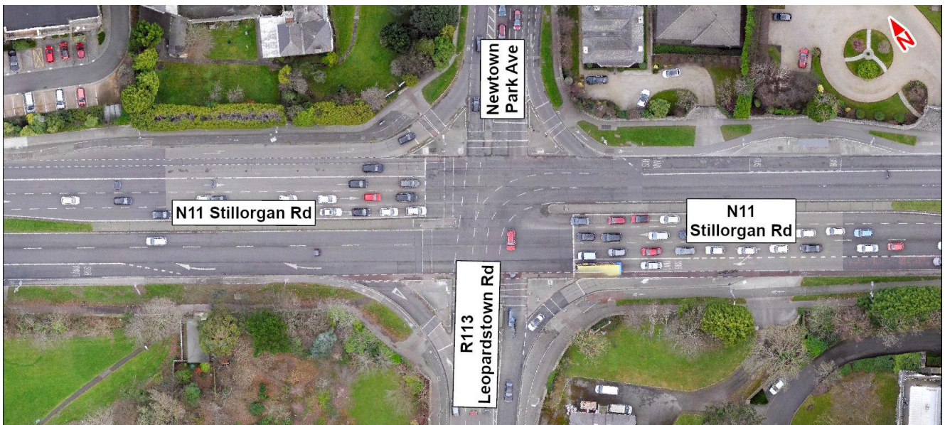
Image 6.27: N11 Stillorgan Road / R113 Leopardstown Road Four-Arm Signalised Junction
