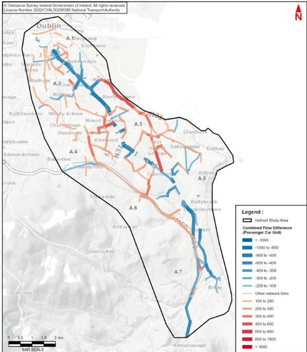
Diagram 6.26: Flow Difference on Road Links (DoMinimum vs. DoSomething), AM Peak Hour, 2028 Opening Year
