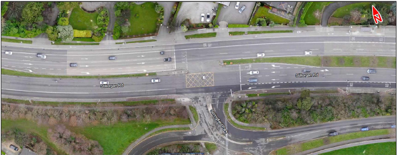
Image 6.28: N11 Stillorgán Road / Springfield Park Three-Arm Signalised Junction
