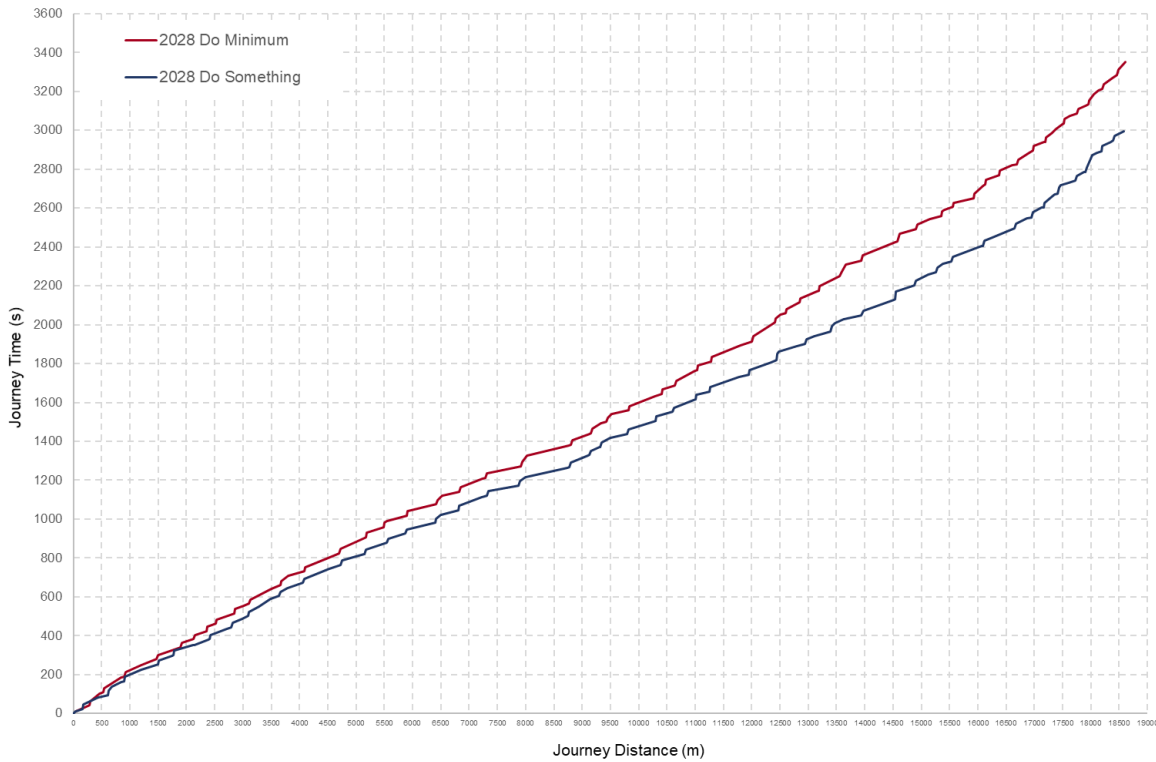
Diagram 6.15: E1 Bus Journey Time (2028 AM, Inbound)
