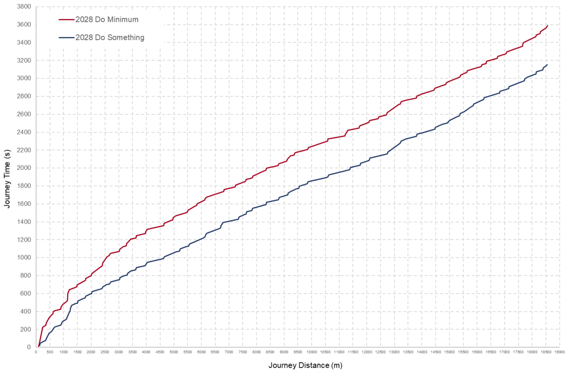
Diagram 6.21: E1 Bus Journey Time (2028 PM, Outbound)
