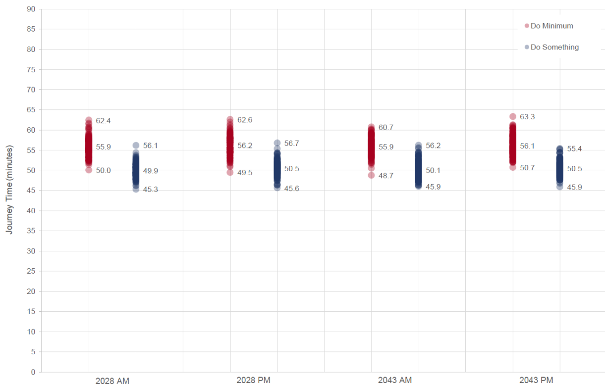
Diagram 6.14: E1 Bus Journey Times (Inbound Direction)
