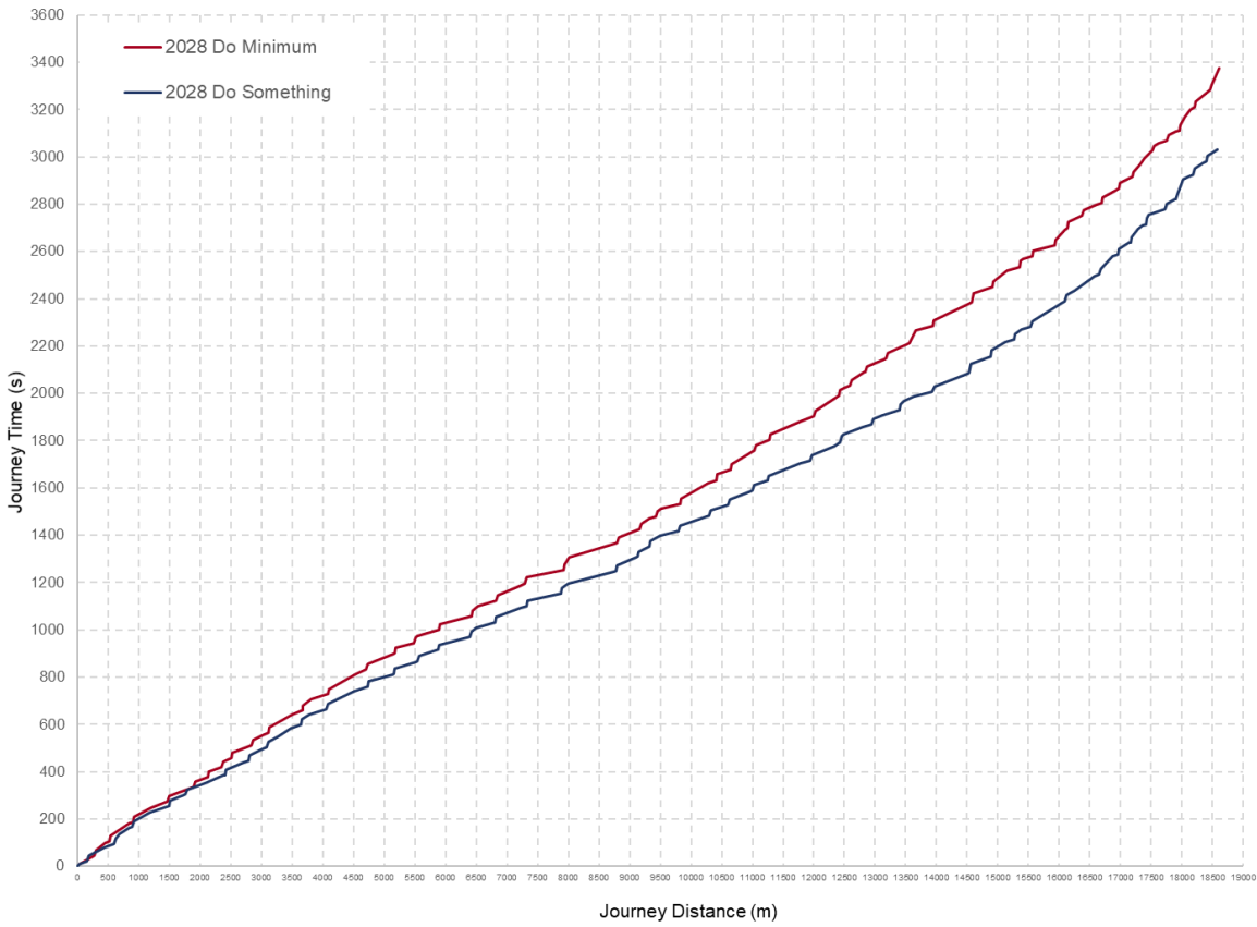
Diagram 6.16: E1 Bus Journey Time (2028 PM, Inbound)
