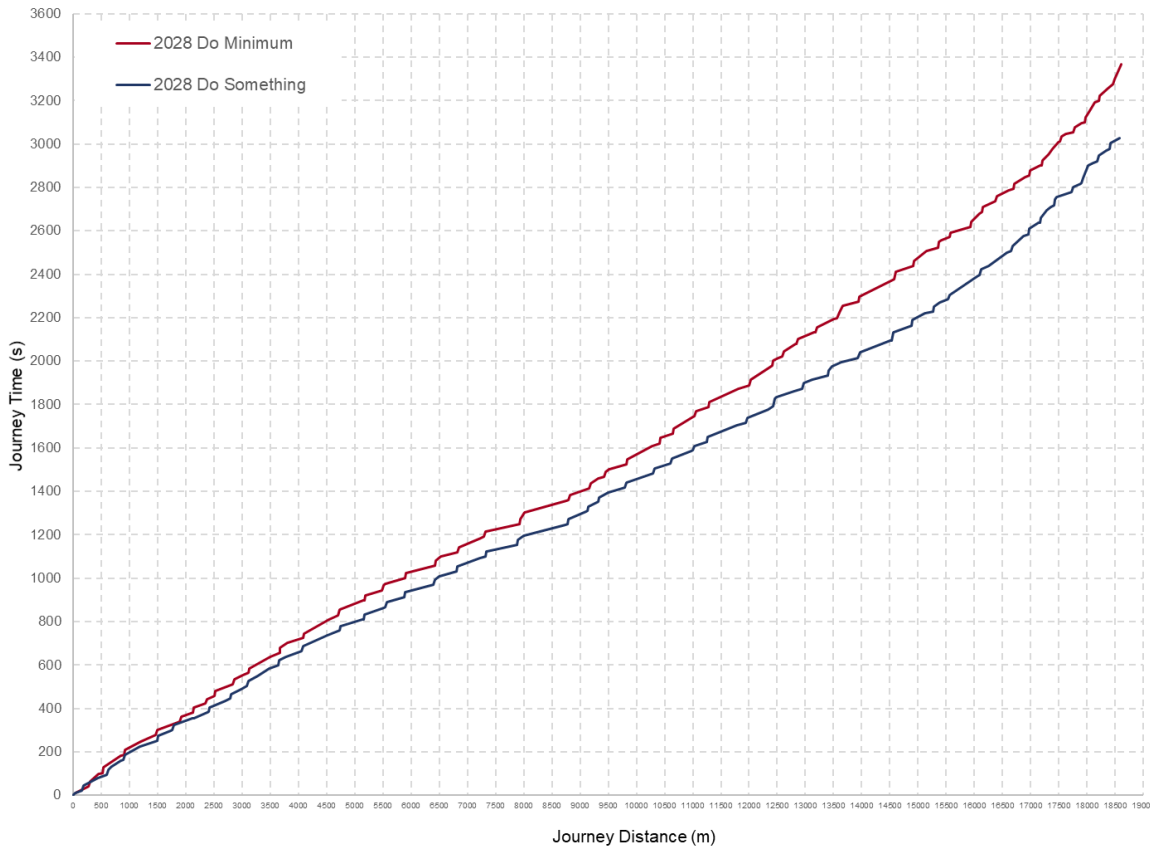
Diagram 6.18: E1 Bus Journey Time (2043 PM, Inbound)
