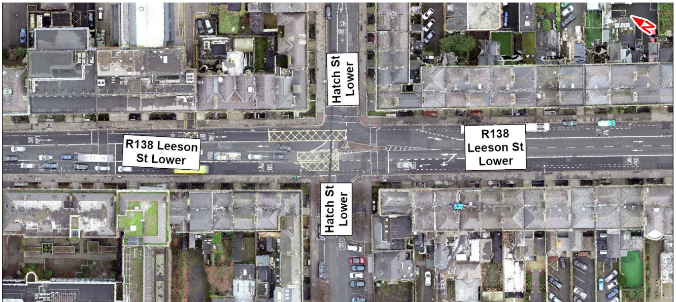
Image 6.2: R138 Leeson Street Lower / Hatch Street Lower Four-Arm Signalised Junction
