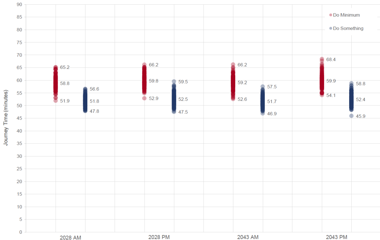
Diagram 6.19: E1 Bus Journey Times (Outbound Direction)
