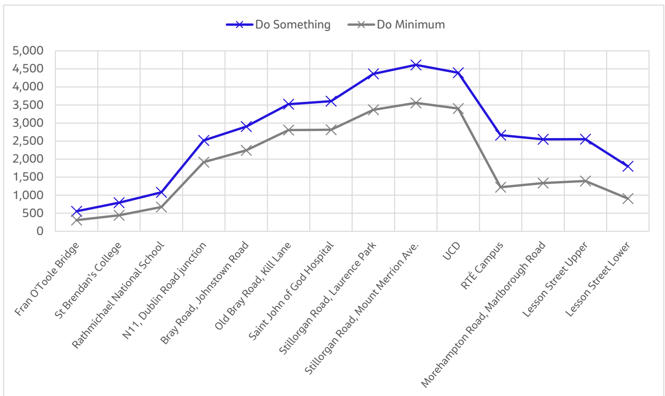
Diagram 6.10: 2028 AM Peak Hour Passenger Volume Along Proposed Scheme (Inbound Direction)
