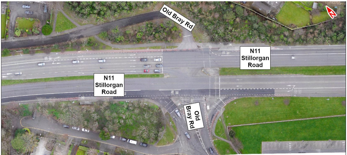
Image 6.31: N11 Bray Road / R842 Old Bray Road Four-Arm Signalised Junction
