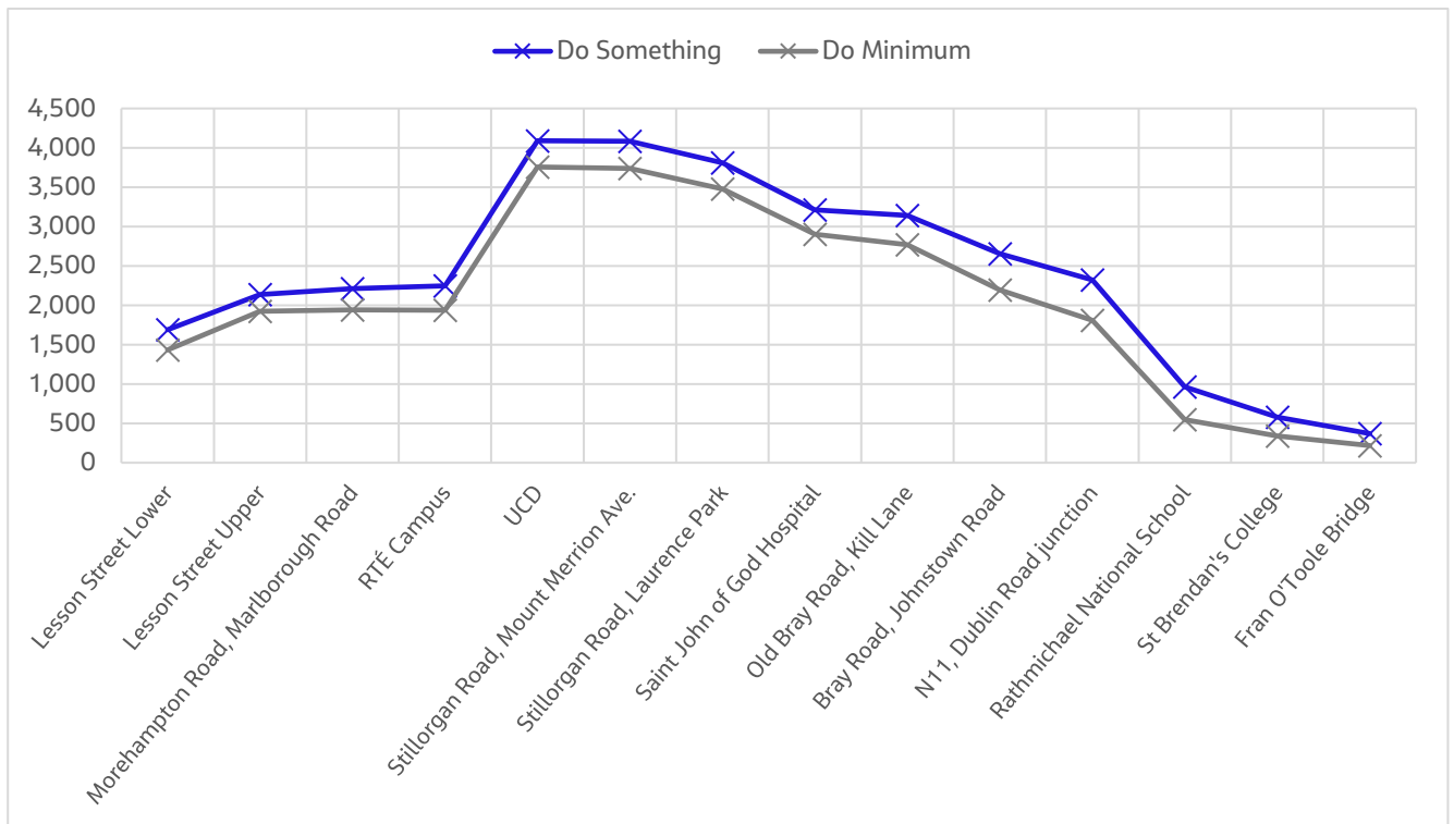
Diagram 6.11: 2028 PM Peak Hour Passenger Volume Along Proposed Scheme (Outbound Direction)
