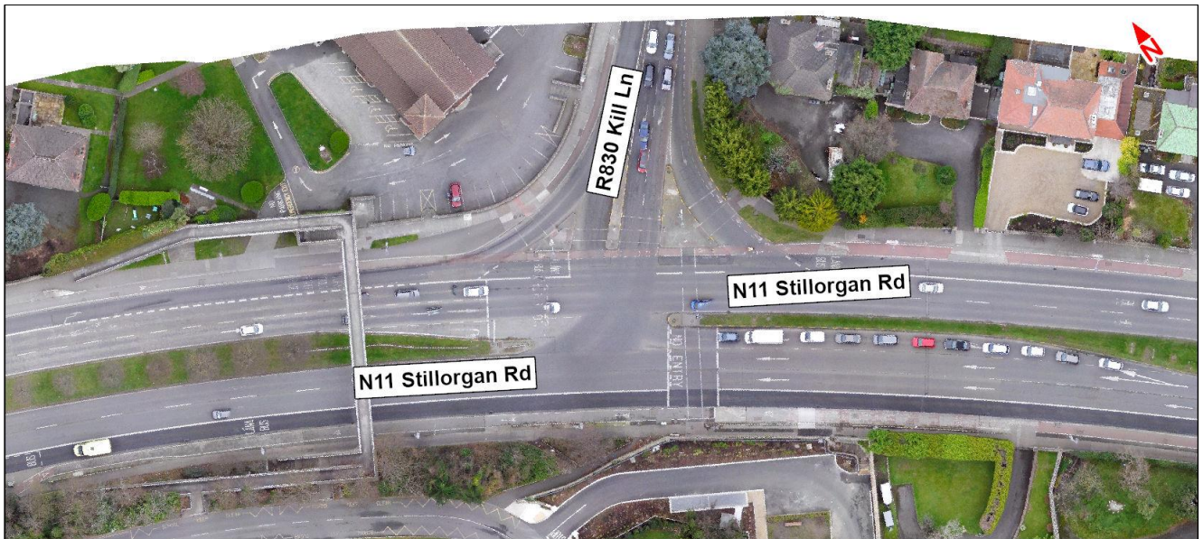
Image 6.29: N11 Stillorgan Road / R830 Kill Lane Three-Arm Signalised Junction
