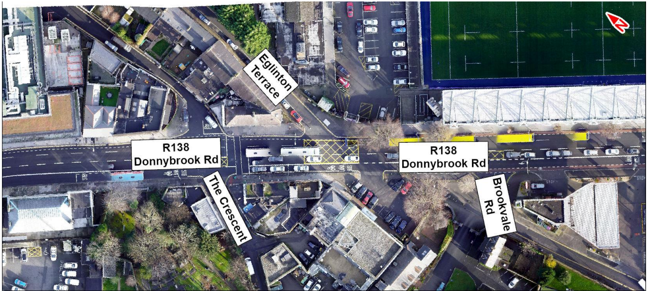
Image 6.13: R138 Donnybrook Road / Eglinton Terrace Priority T-Junction
