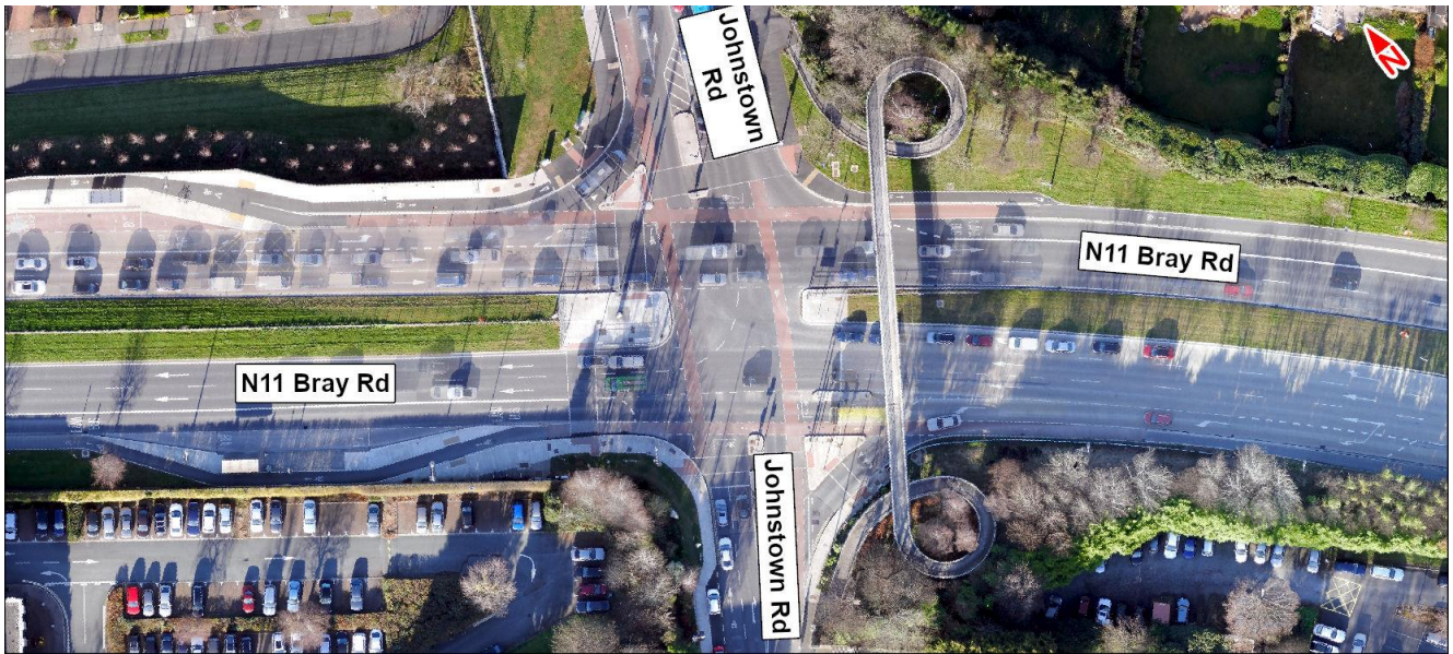
Image 6.33: N11 Bray Road / Johnstown Road Four-Arm Signalised Junction
