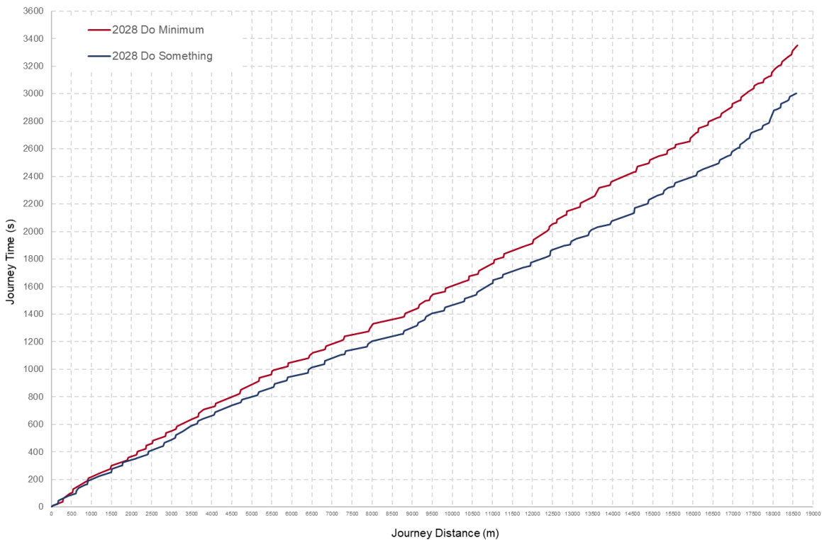
Diagram 6.17: E1 Bus Journey Time (2043 AM, Inbound)
