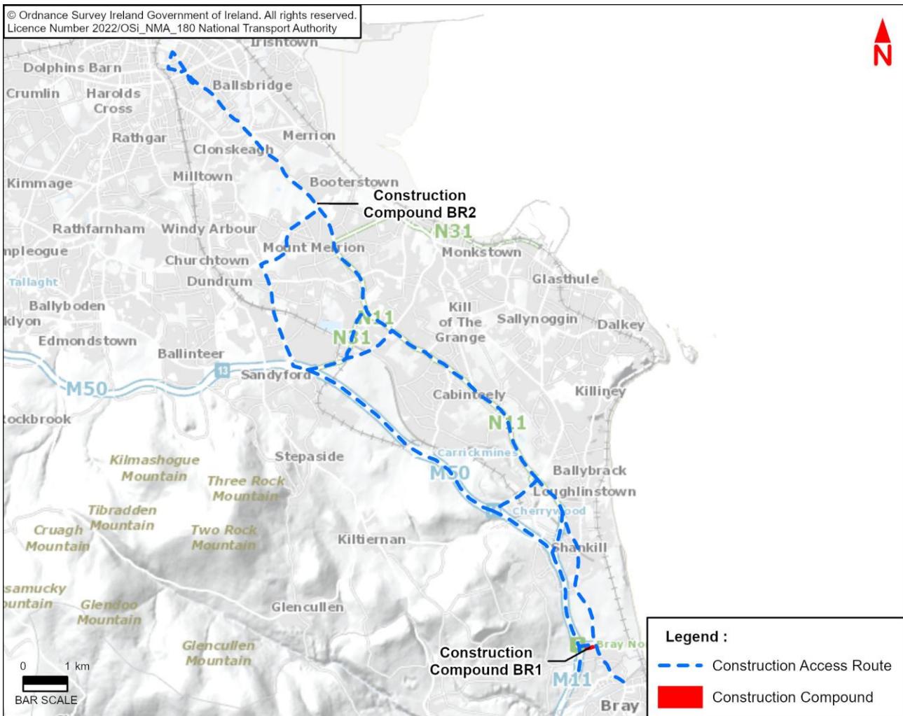
Diagram 6.5: Proposed Construction Routes and Main Compound Locations
